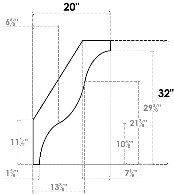
SIDE PROFILE
